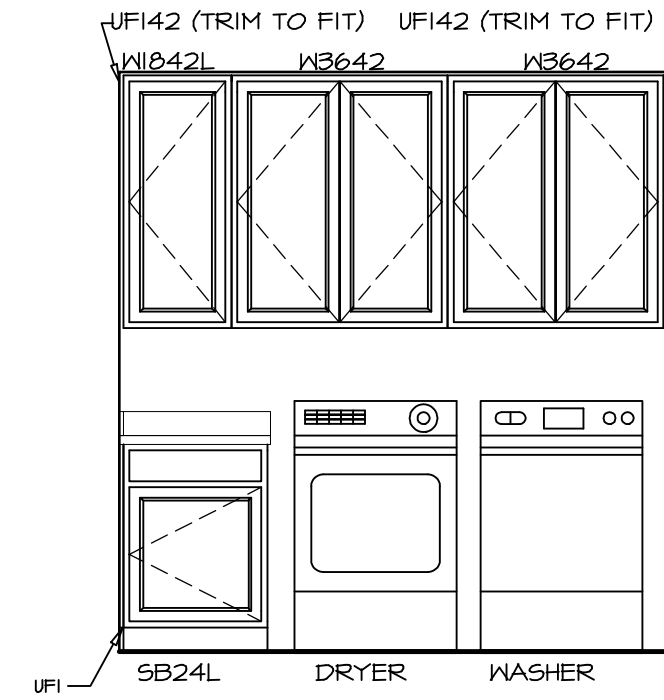
ELEVATION "M"
