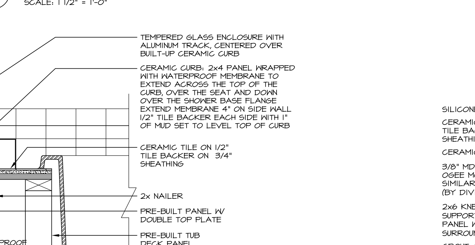
6 SECTION OF SHOWER SEAT AND SHELF SCALE: 1/2" = 1'-0"
