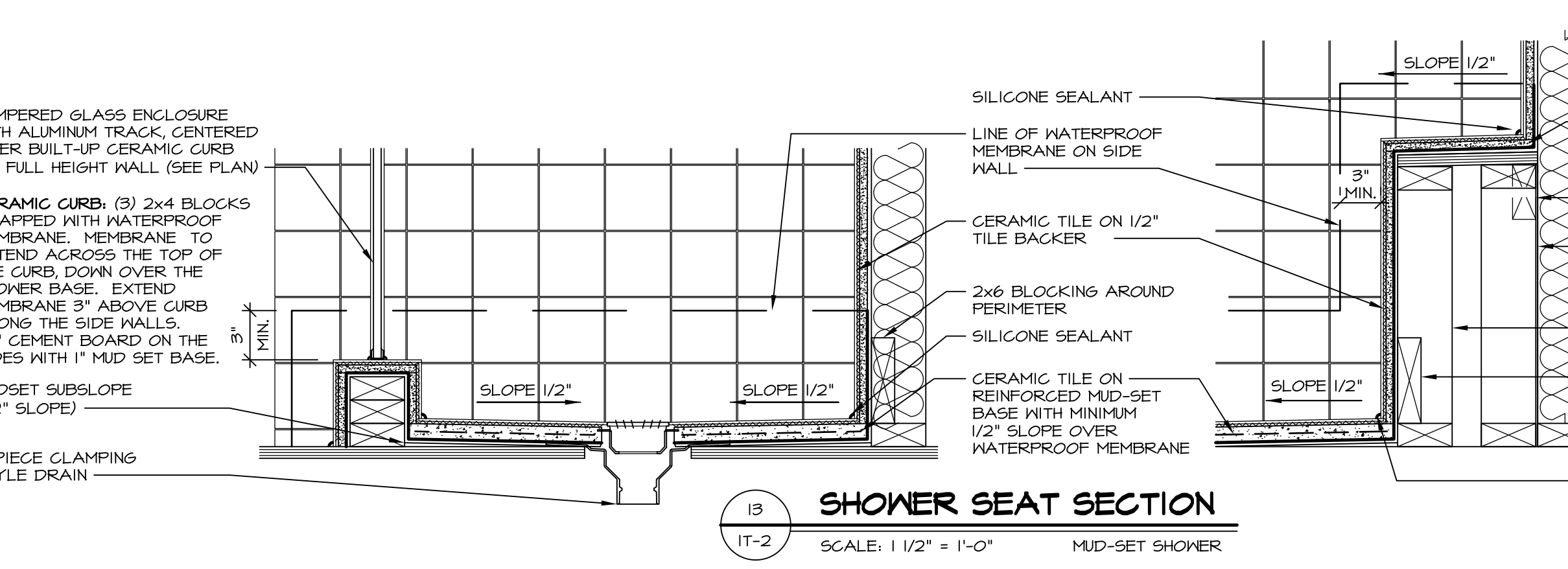
14 SHOWER SEAT SECTION SCALE: 1-1/2" = 1'-0" MUD-SET SHOWER
