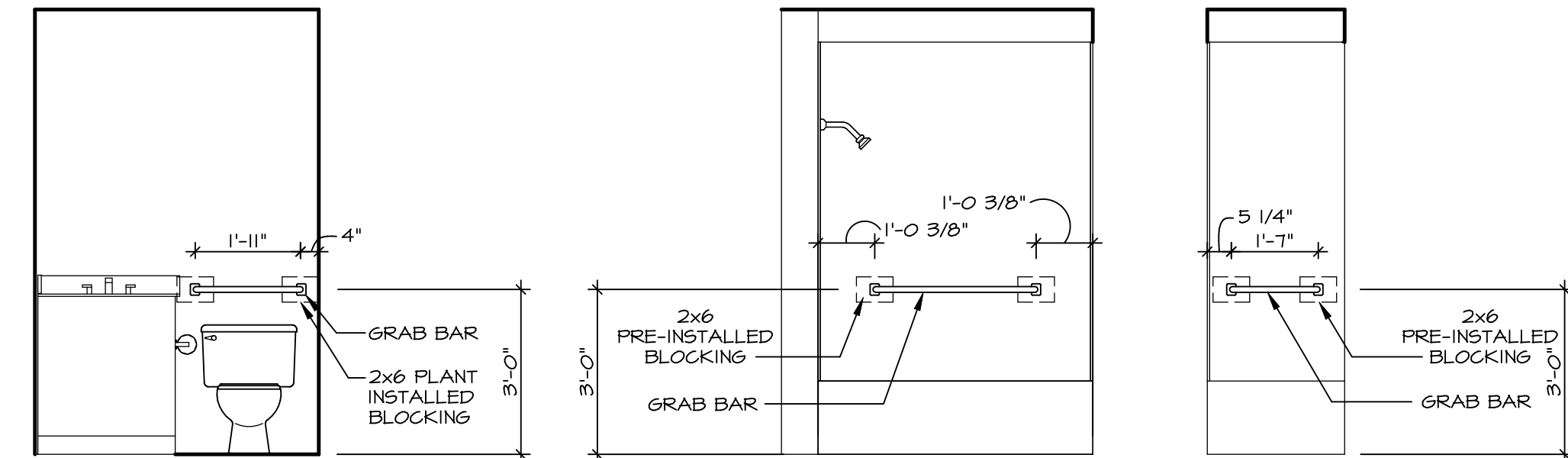
2 BATH #1 - BLOCKING DETAIL SCALE: 3/8" = 1'-0"
