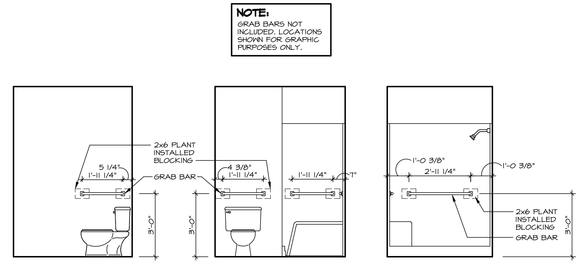
I OWNER'S BATH - BLOCKING DETAIL SCALE: 3/8" = 1'-0"
