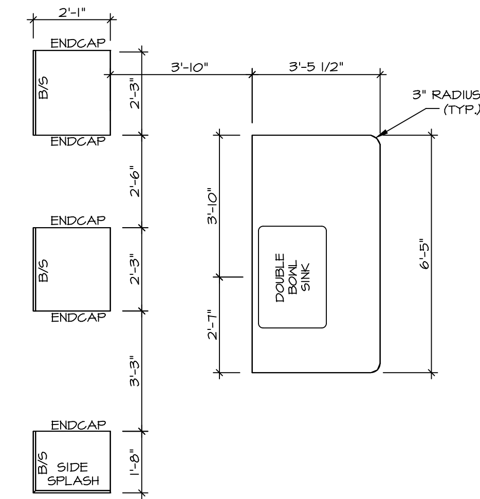
KITCHEN COUNTERTOP PLAN / KC-343I
