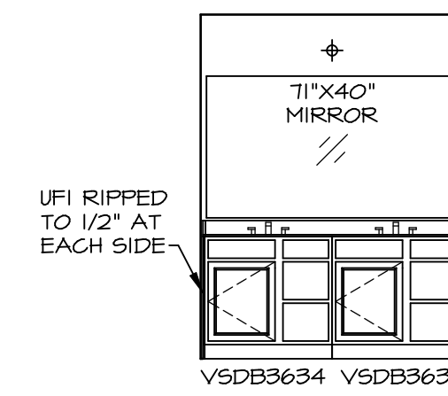
J OWNER'S BATH SCALE: 1/4" = 1'-0" OWNER'S BATHROOM SHOWER "AMA"
