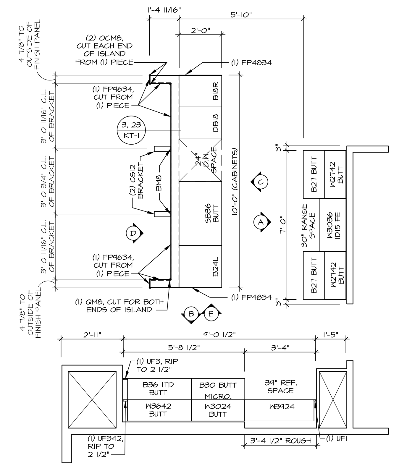
1 KITCHEN CABINET LAYOUT KC-3521 A-12 SCALE: 3/8" = 1'-0" APPLIANCE LAYOUT W/ RANGE "KAA"
