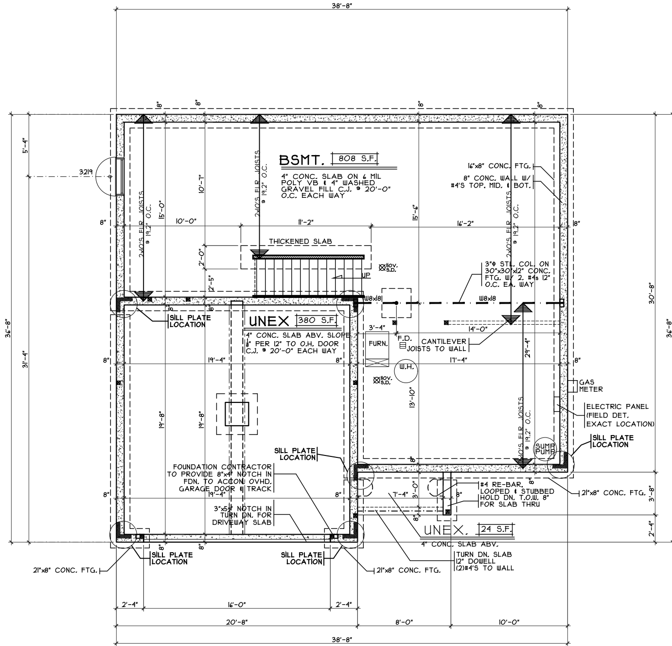
FOUNDATION PLAN
