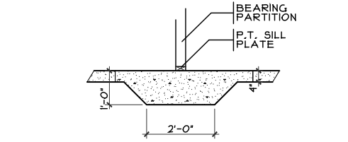
THICKENED SLAB
