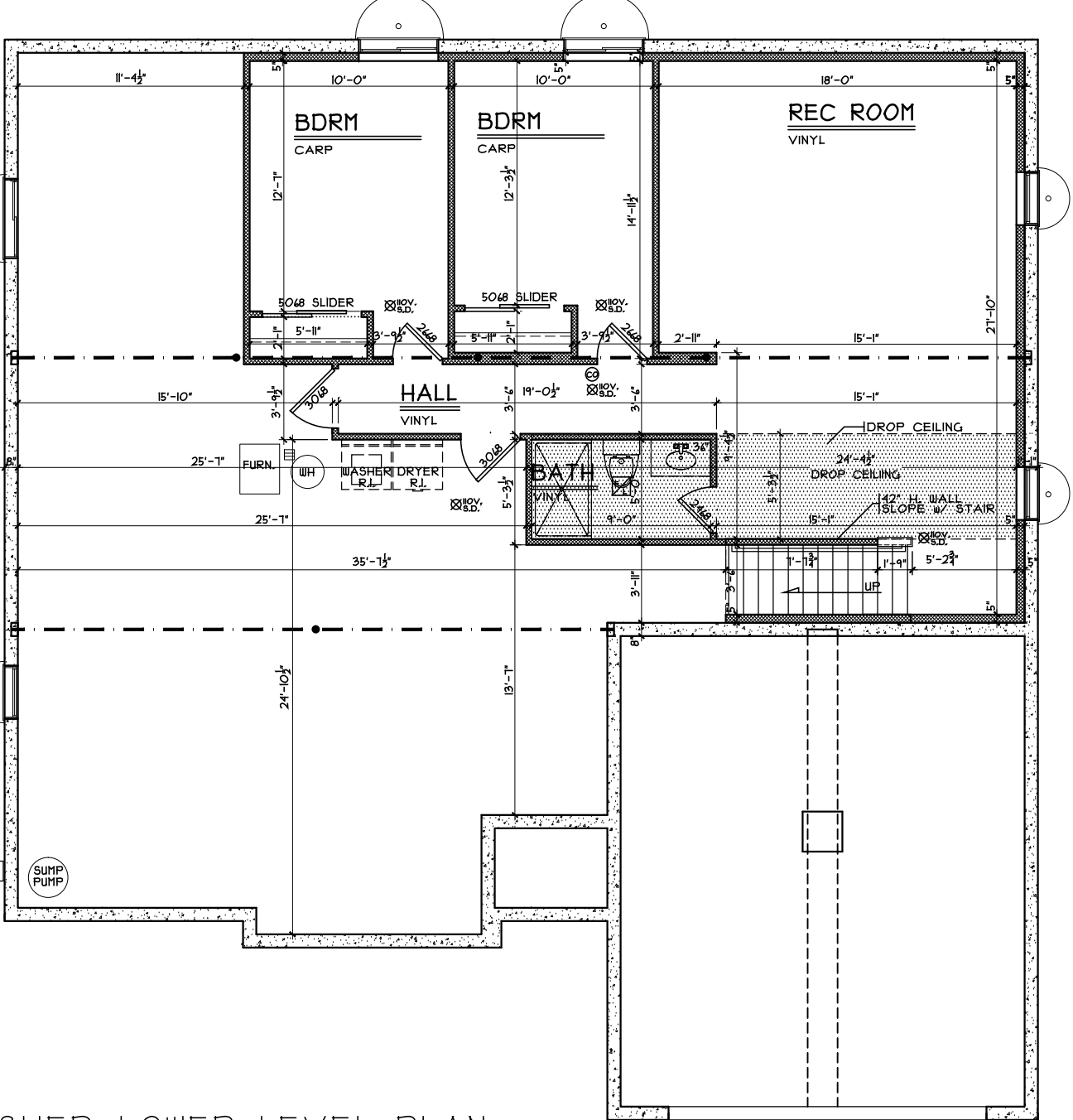
FINISHED LOWER LEVEL PLAN
