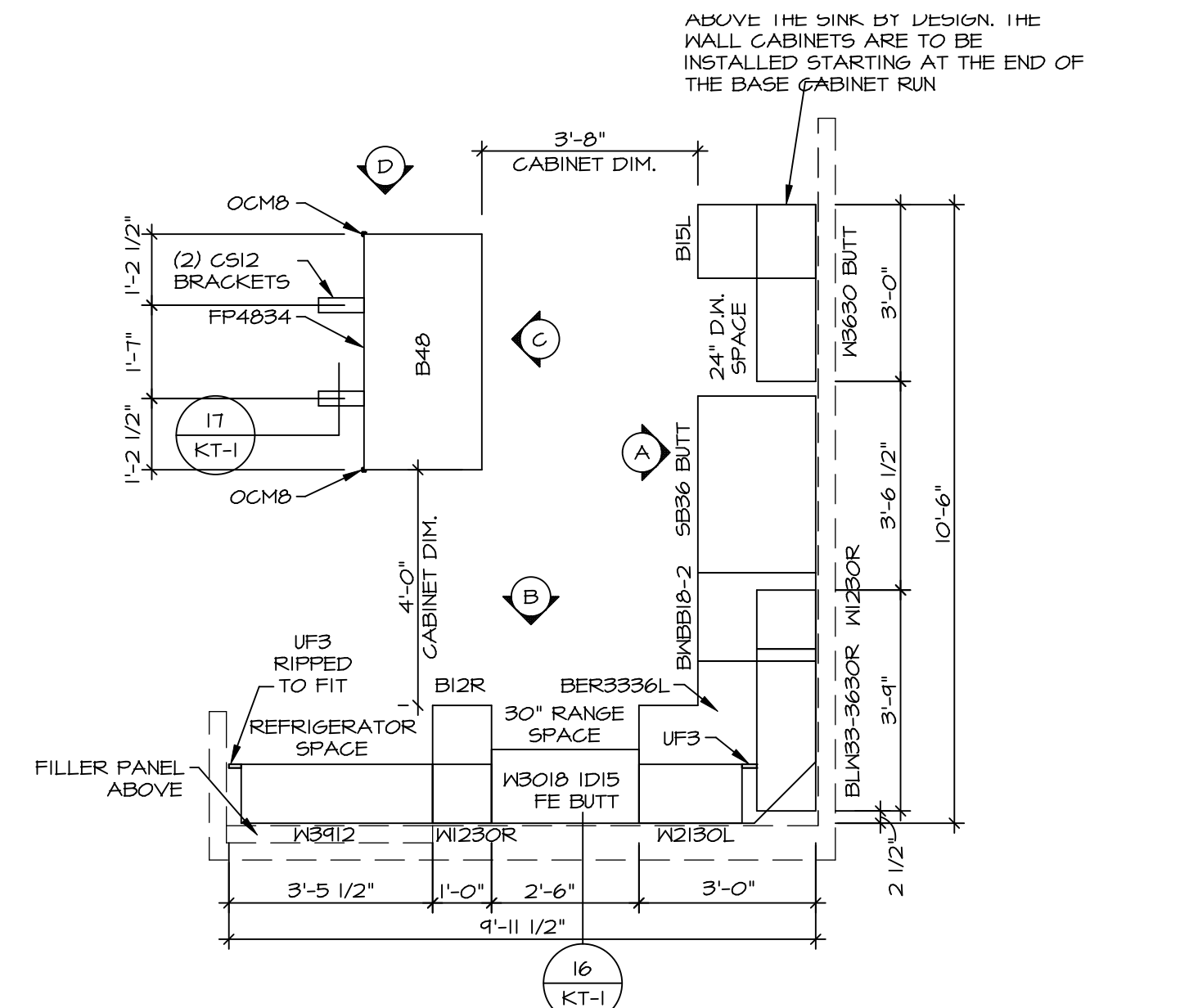
KITCHEN CABINET PLAN / KC-3765 SCALE: 3/8" = 1'-0" A-II
