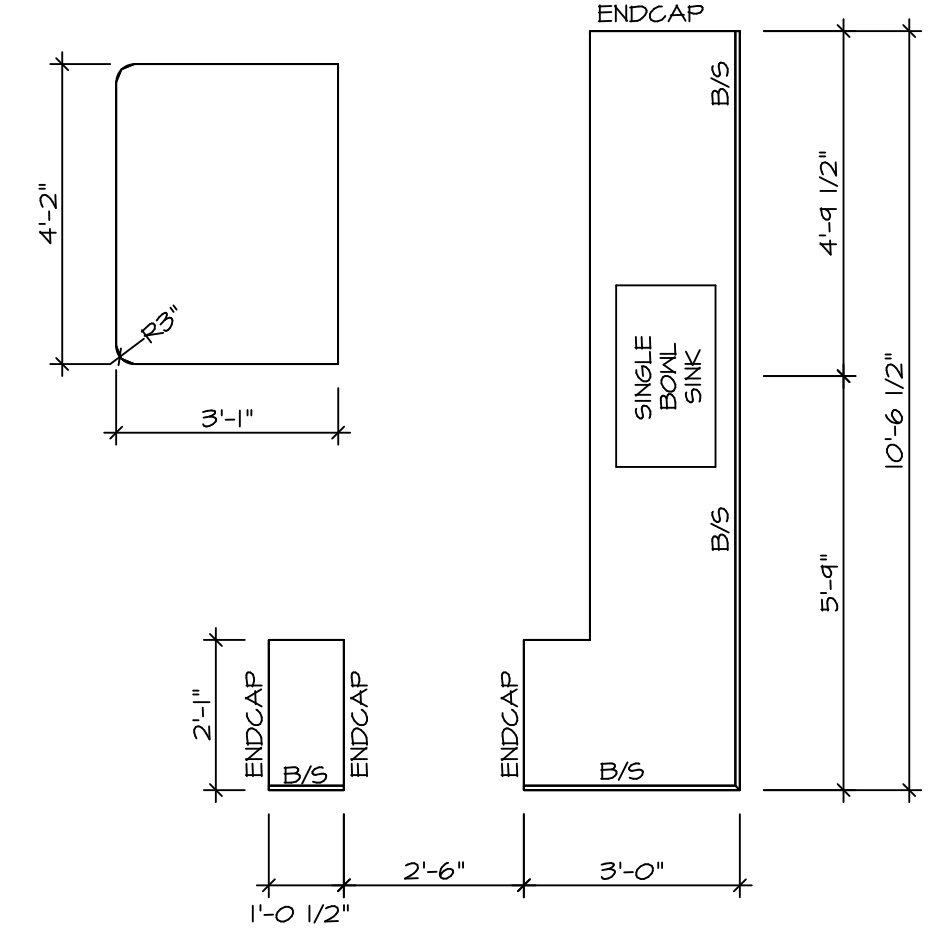
KITCHEN COUNTERTOP PLAN KC-3765 SCALE: 3/8" = 1'-0" A-II
