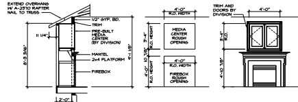
4 OPT. ENTERTAINMENT ALCOVE SCALE: 1/4" = 1'-0"
