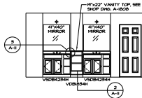
B OWNER'S BATH SCALE: 1/4" = 1'-0"
