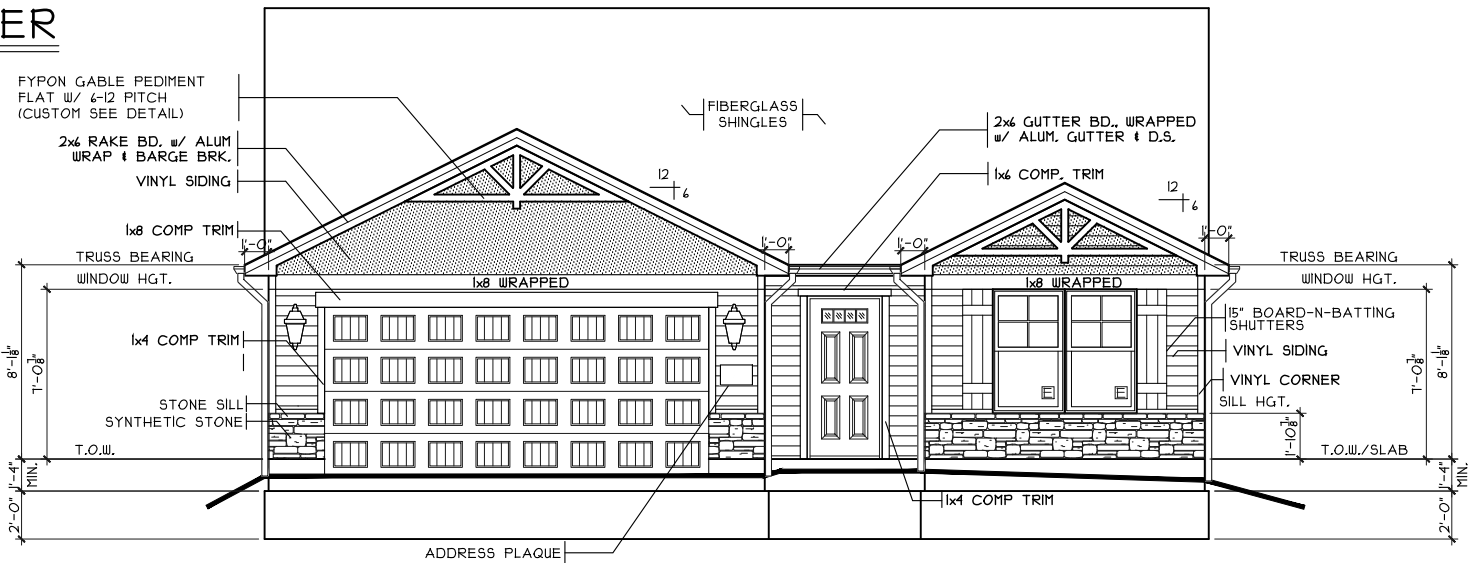
FRONT ELEVATION
