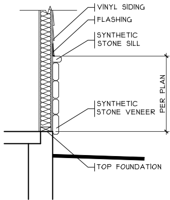
STONE BASE DETAIL
