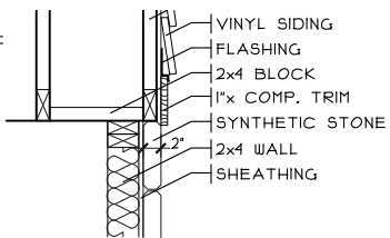
STONE DETAIL
