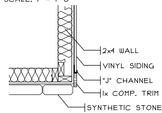
STONE/VINYL CORNER
