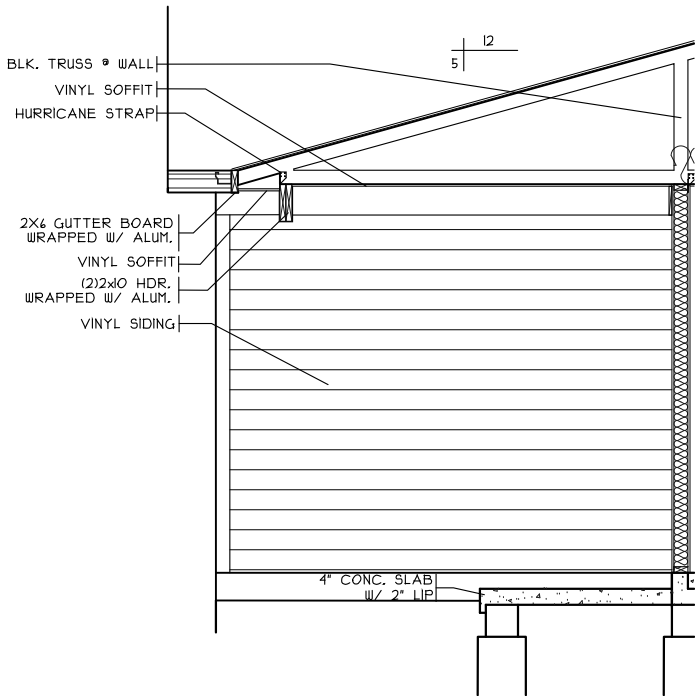
PORCH DETAIL
