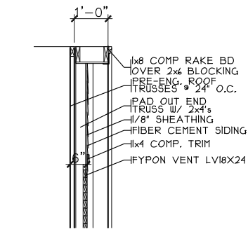
LOUVER VENT DETAIL
