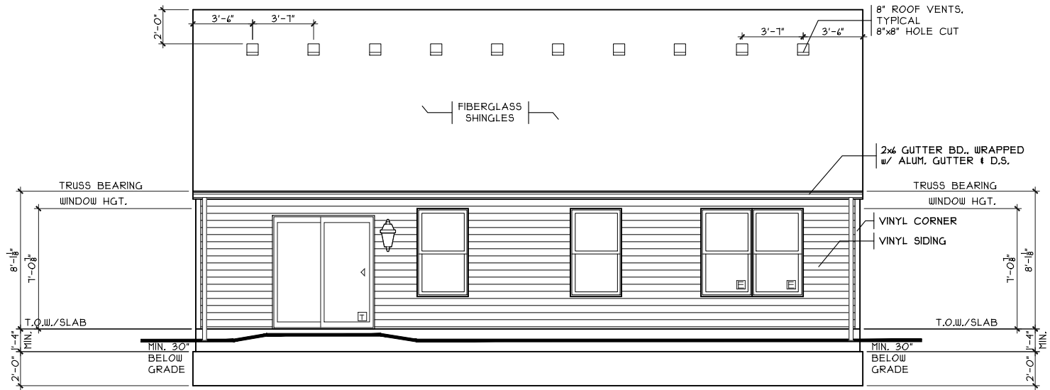
REAR ELEVATION
