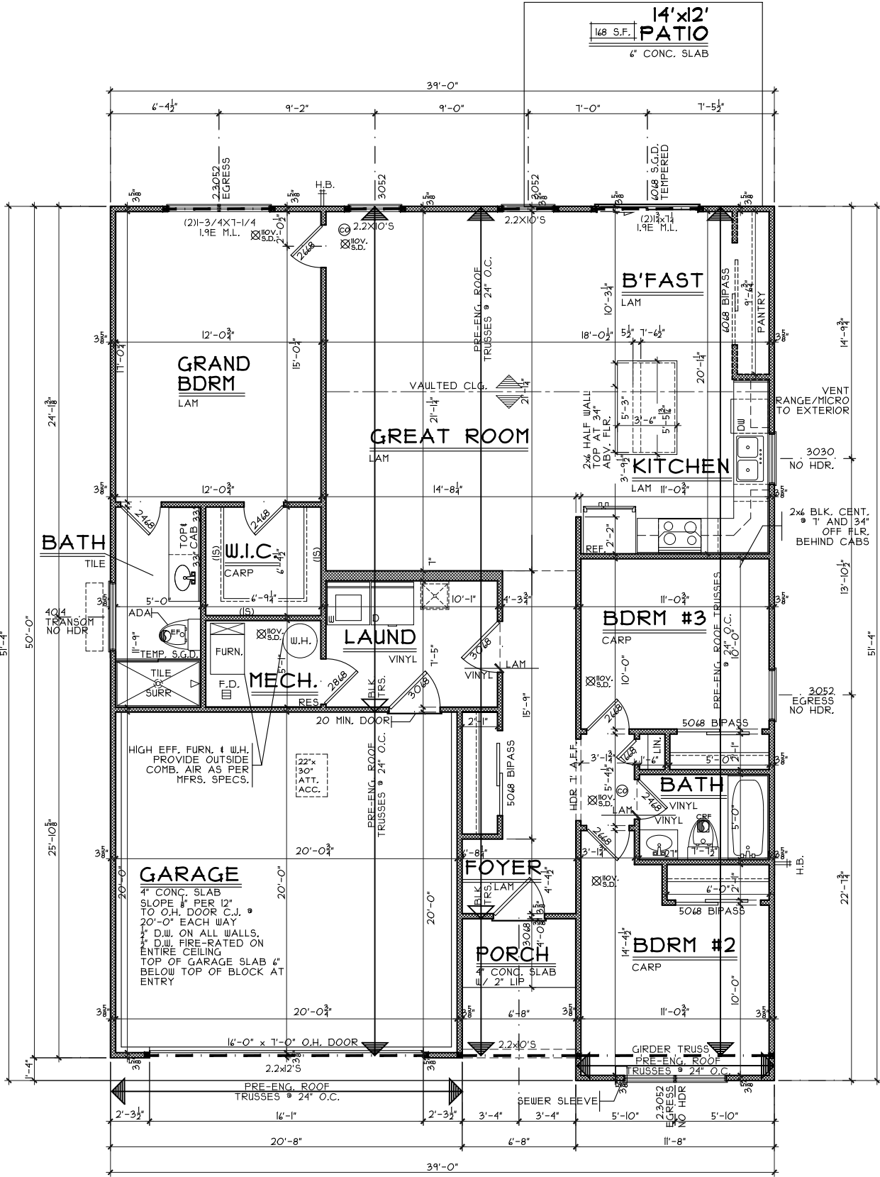
FIRST FLOOR PLAN SCALE: 1/8" = 1'-0" 1500 S.F
