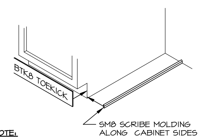
NOTE: OMIT SMO SCRIBE MOLDING AT DISHWASHER SPACES. TOEKICK / SCRIBE DETAIL SCALE: 3/4" = 1'-0" A-II
