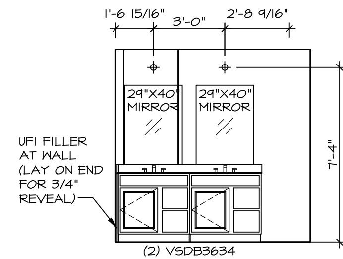
P OWNERS BATH SCALE: 1/4" = 1'-0" OWNER'S BATHROOM SOAKING TUB AND SHOWER GLASS SURROUND "AMF" NEW LIGHT/MIRROR LAYOUT DBL. VANITY "AFE"
