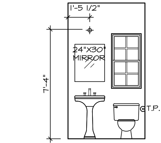
C POWDER ROOM SCALE: 1/4" = 1'-0" CRAFTSMAN SPECIFICATIONS "SZC"
