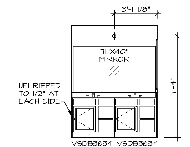
L OWNER'S BATH SCALE: 1/4" = 1'-0" OWNER'S BATHROOM W/ ROMAN SHOWER *AM6*
