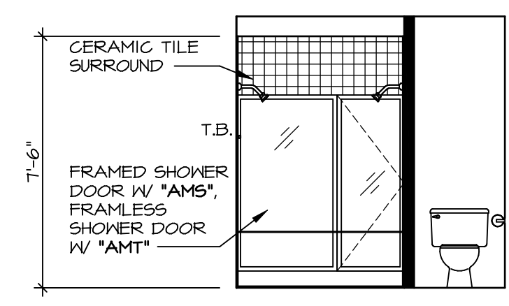
K OWNER'S BATH SCALE: 1/4" = 1'-0" OWNER'S BATHROOM W/ ROMAN SHOWER *AM6*
