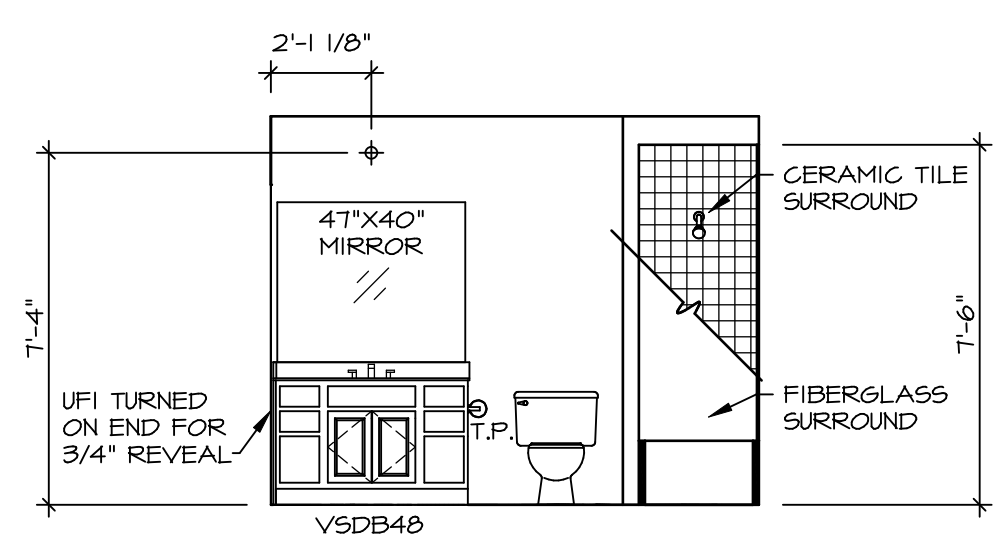
F BATH #1 SCALE: 1/4" = 1'-0" SINGLE BOWL VANITY *VC*
