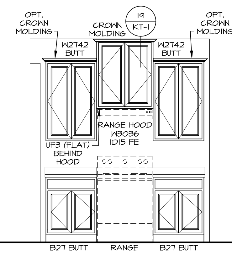
CABINET ELEVATION A
