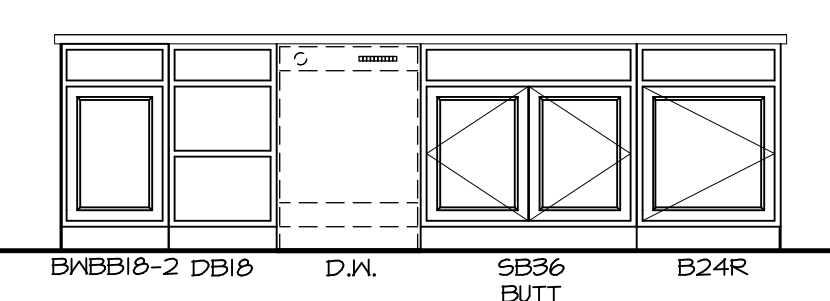
CABINET ELEVATION C
