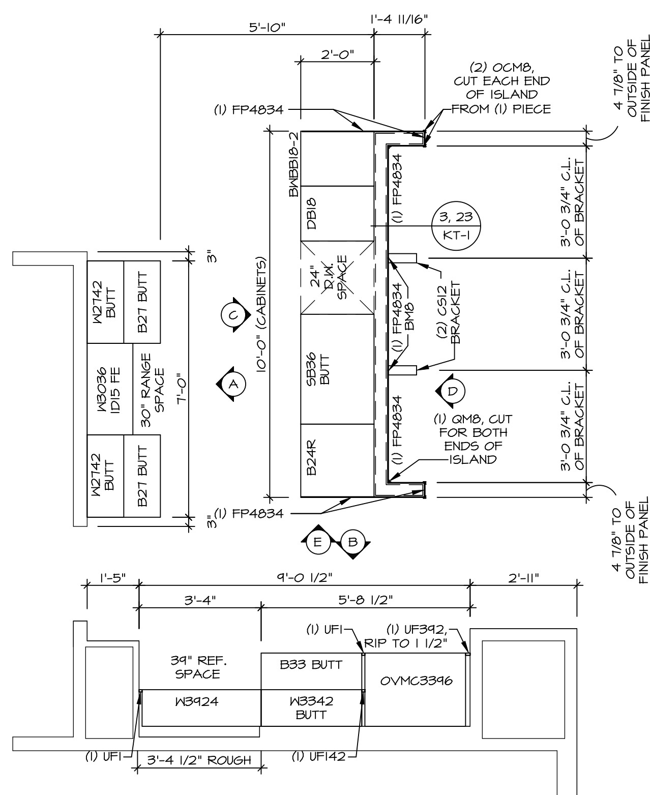
KITCHEN CABINET LAYOUT KC-3522(TC)
