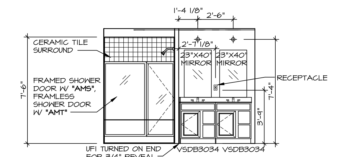
M OWNER'S BATH SCALE: 1/4" = 1'-0"
